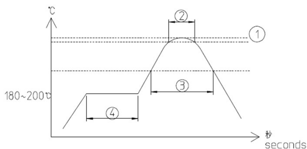
Fig2. Reflow Profile
