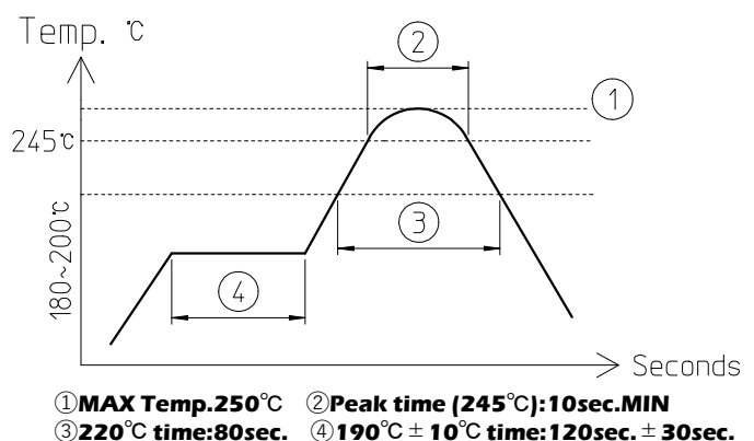
Fig 2. Reflow Profile
